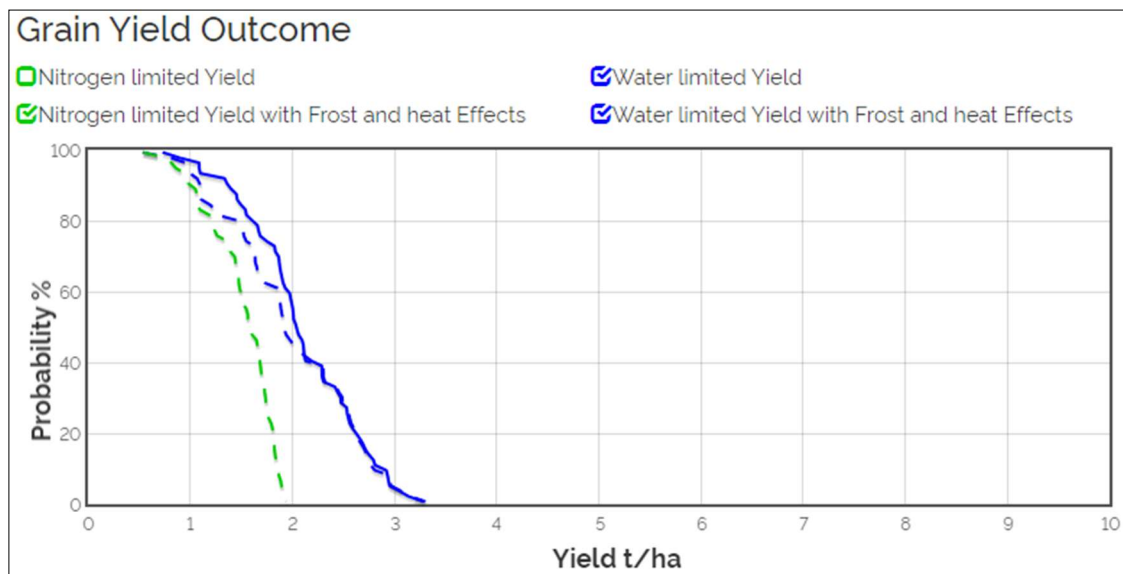
Figure 1: Yield Prophet graph from Lock, generated on 15 April 2024. Green line indicates the predicted nitrogen limited yield and blue line indicates the water limited yield. The dotted blue line represents water limited yield potential with frost and heat effects. This is based on the assumption that yield is only limited by these factors and no others (ie pests, weeds, diseases).
